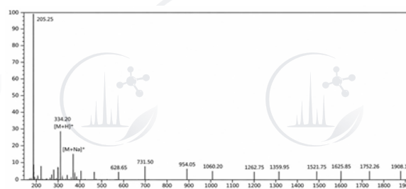
FIGURE 2 — MASS SPECTROMETRIC DATA (LC-MS/MS)
