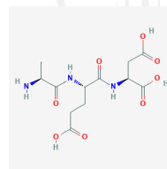
MOLECULAR STRUCTURE
