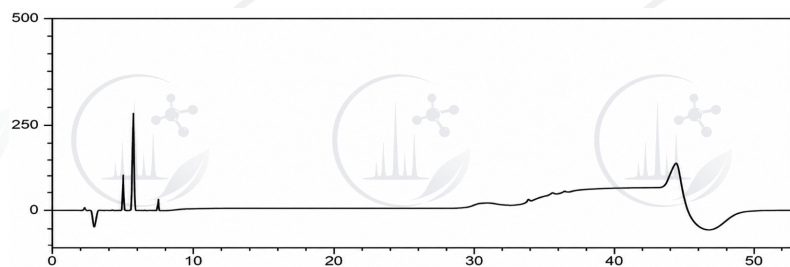
FIGURE 1 — CHROMATOGRAPHIC DATA (HPLC-UV)
