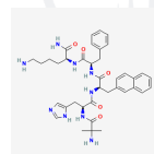
MOLECULAR STRUCTURE
